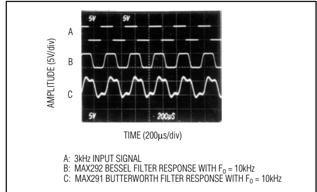
Figure 1. Bessel vs. Butterworth Filter Responses
